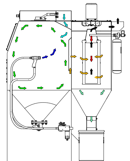
▼ Injector blast principle
